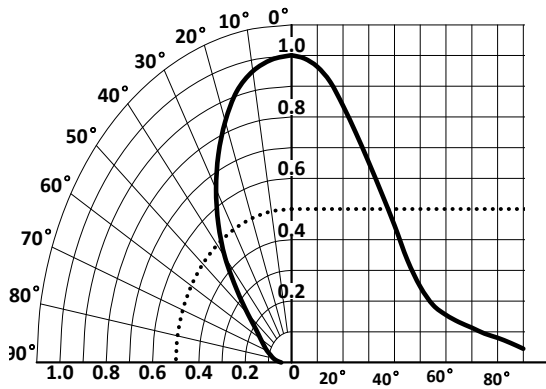
Typical Polar Radiation Plot - B80
