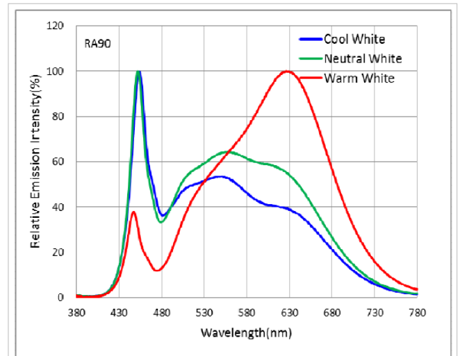
COLOR SPECTRUM ( R_a \geq 90 T_j = 25^\circ\text{C} )
