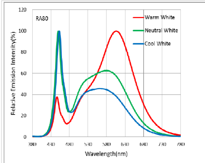
COLOR SPECTRUM ( R_a \geq 80 T_j = 25^\circ\text{C} )
