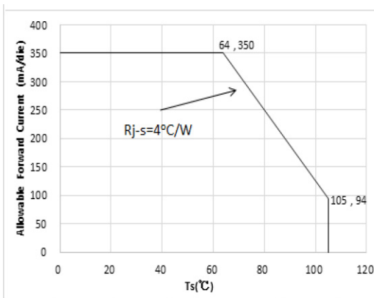
MAX FORWARD CURRENT VS. SOLDERING TEMP.
