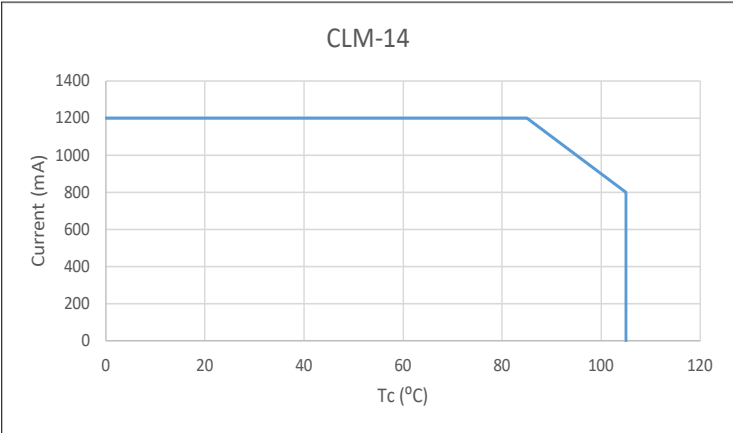
Derating Curves
