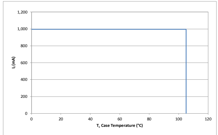
Derating Curve
