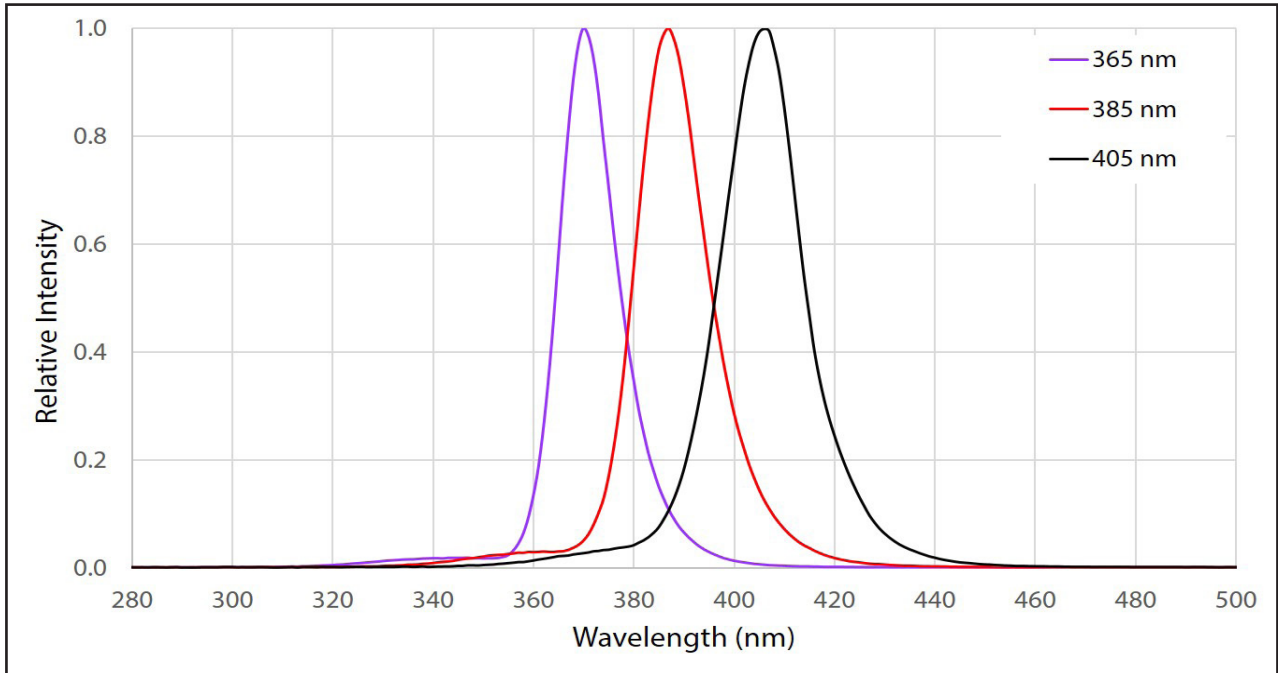
Typical Spectrum 10
