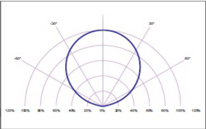
Viewing Angle Distribution(Tj = 25°C)
