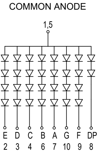
CIRCUIT DIAGRAM
