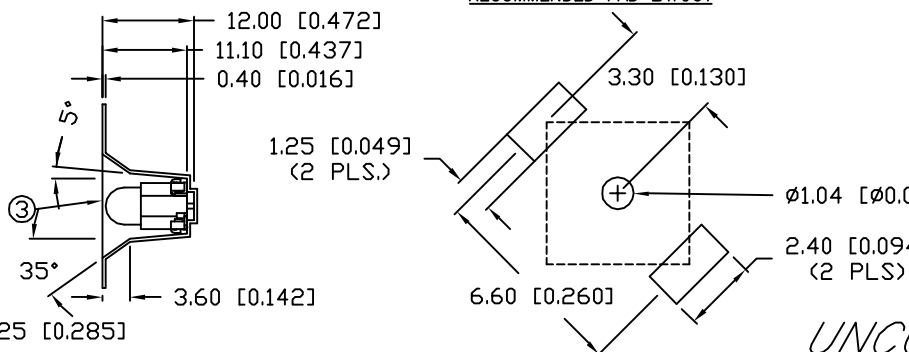
RECOMMENDED PAD LAYOUT
