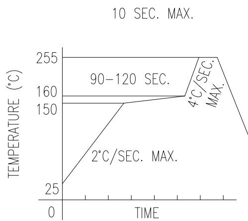
LEAD FREE REFLOW PROFILE
