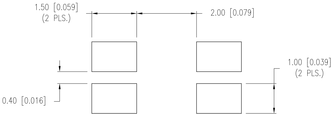
RECOMMENDED SOLDER PAD LAYOUT
