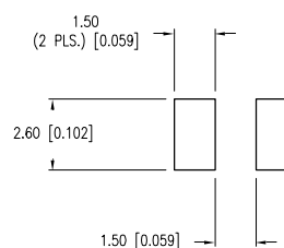
A RECOMMENDED SOLDER PAD LAYOUT
