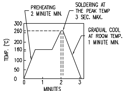
REFLOW PROFILE
