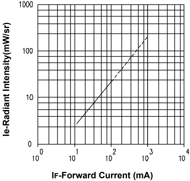
Relative Intensity vs. Forward Current
