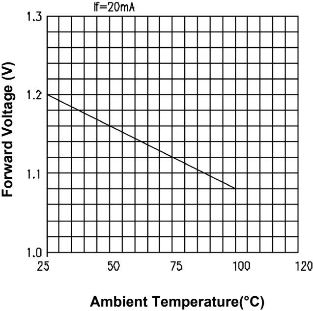
Forward Voltage vs. Ambient Temperature(°C)
