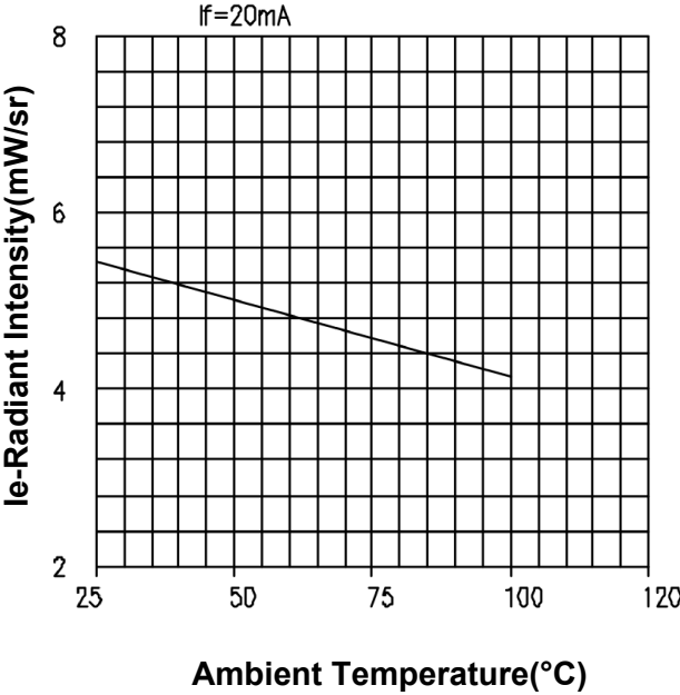
Relative Intensity vs. Ambient Temperature(°C)
