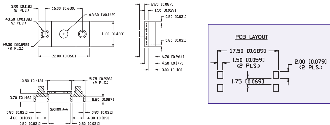
Figure 36 Part # LPA-C021301S-2
