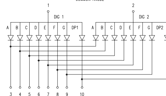
COMMON ANODE
