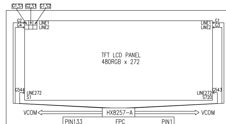
BLOCK DIAGRAM
