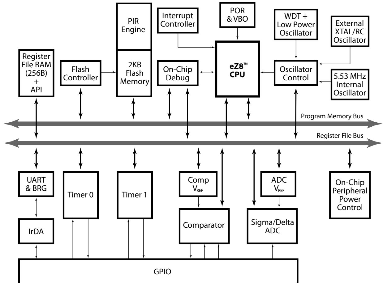
Figure 1. Z8FS021 MCU Block Diagram
