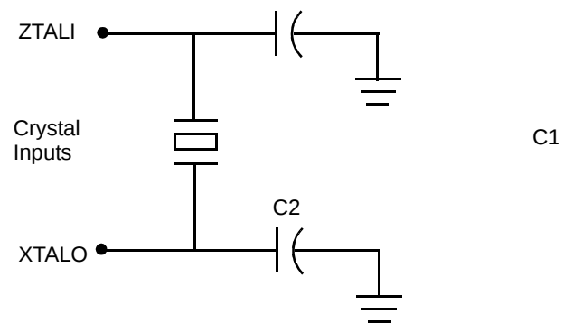
Figure 8. Crystal Connection
