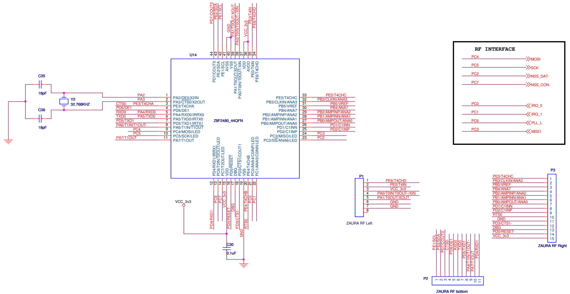
Figure 10. ZAURA RF Wireless 915MHz Module, #1 of 2
