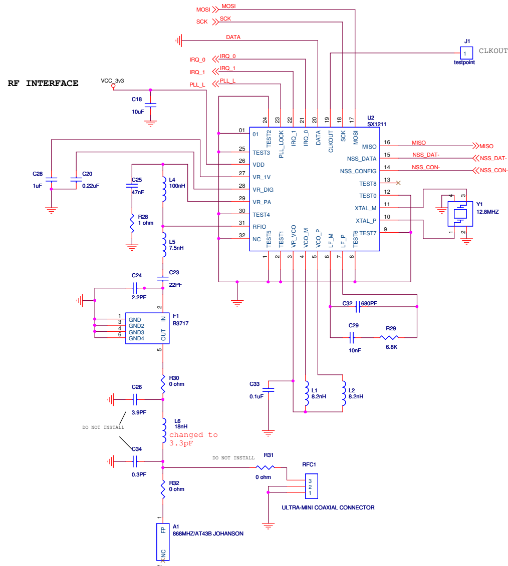
Figure 8. ZAURA RF Wireless 868MHz Module, #1 of 2
