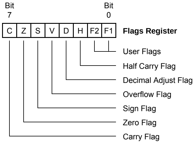
Figure 53. Flags Register
