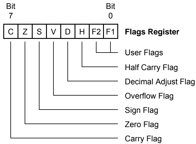
Figure 53. Flags Register
