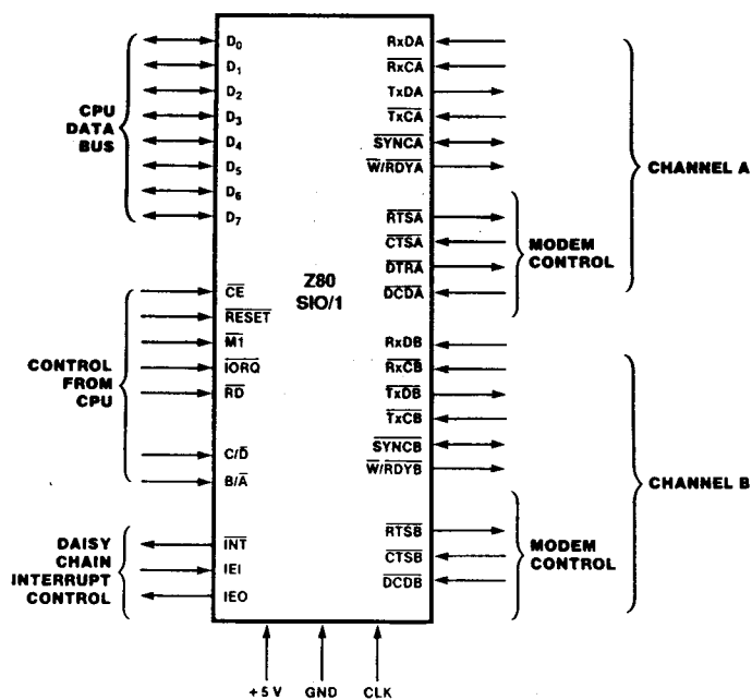
Figure 3. Pin Functions
