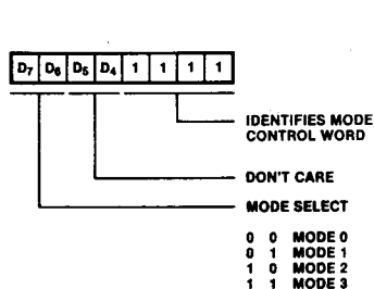
Figure 6. Mode Control Word
