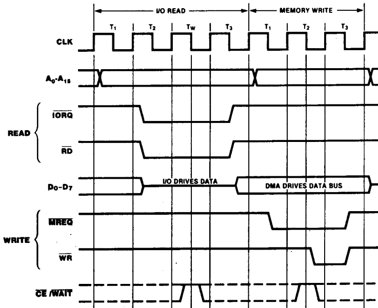
Figure 13. I/O-to-Memory Transfer
