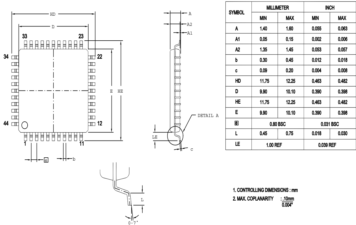
Figure 18. 44-Pin LQFP Package Diagram
