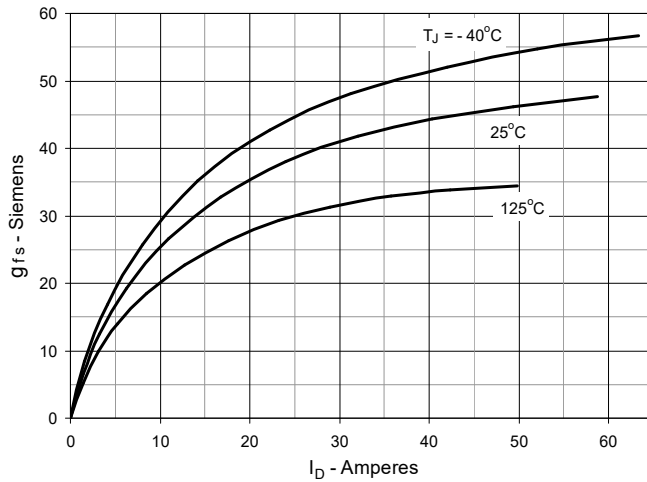
Fig. 9. Transconductance
