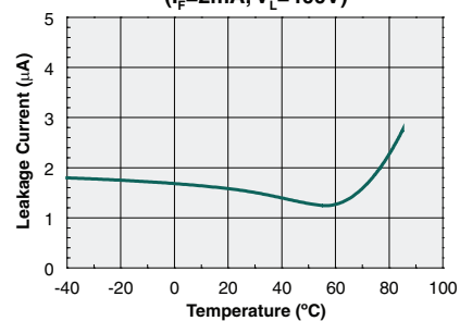
Leakage Current vs. Temperature Measured Across Pins 5&6, 7&8 ( I_F=2\text{mA} , V_L=400\text{V} )
