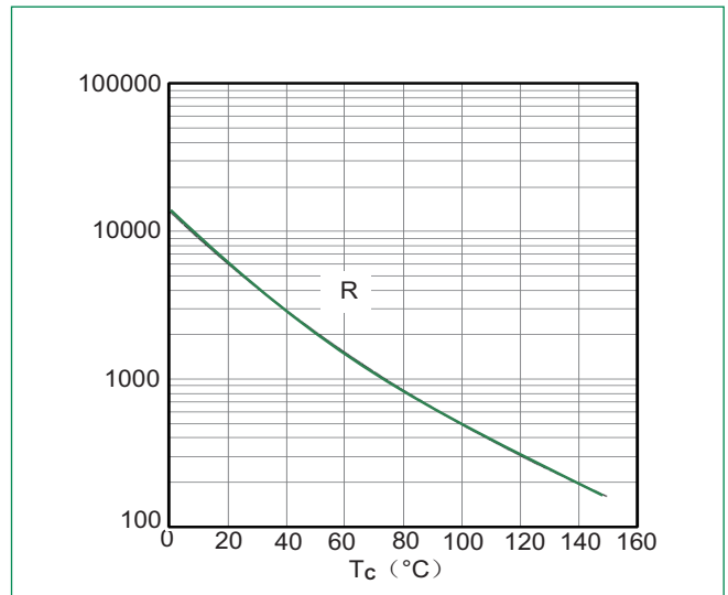
Figure 14: NTC Characteristics
