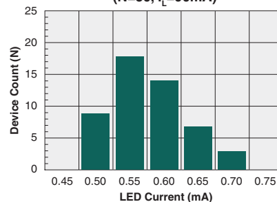
Typical I_F for Switch Dropout (N=50, I_L=90\text{mA} )
