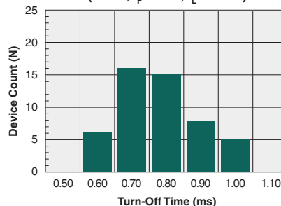
Typical Turn-Off Time (N=50, I_F=5\text{mA} , I_L=90\text{mA} )
