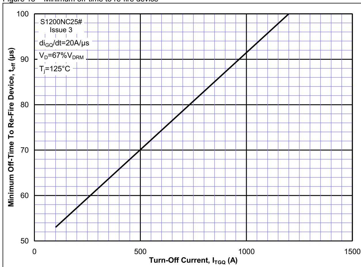
Figure 18 – Minimum off-time to re-fire device
