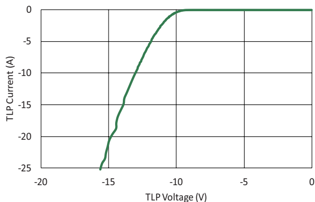
Negative Transmission Line Pulsing (TLP) Plot
