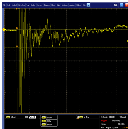
IEC 61000-4-2 -8 kV Contact ESD Clamping Voltage
