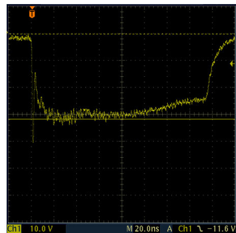
ISO10605 -8 kV Contact ESD Clamping Voltage
