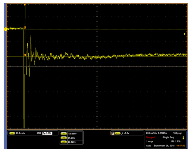
ISO10605 -8 kV Contact ESD Clamping Voltage
