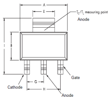
Pad Layout for SOT-223
