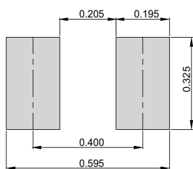
Recommended Soldering Pad Layout (mm)
