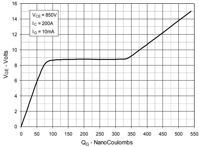
Fig. 7. Gate Charge
