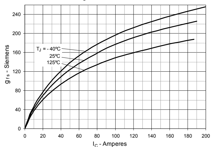
Fig. 6. Transconductance
