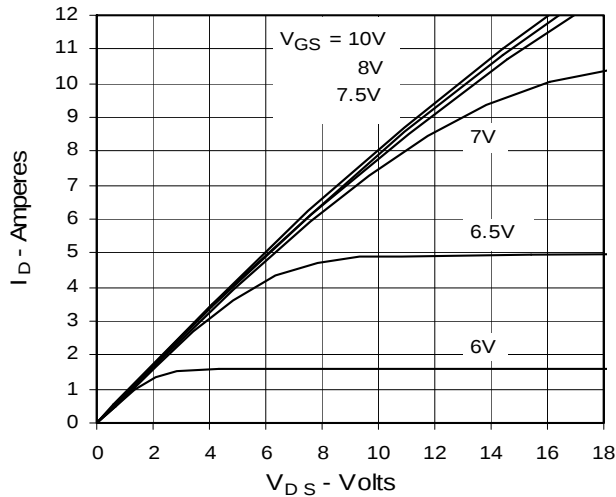
Fig. 3. Output Characteristics
