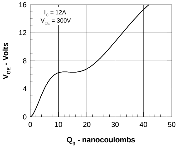
Fig. 9. Gate Charge
