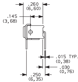
PC MOUNTING
