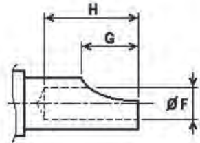
Termination
