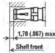
Female contact
