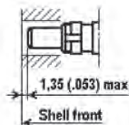
Male contact
