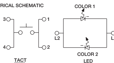
ELECTRICAL SCHEMATIC
