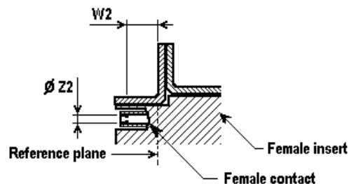
Female connector
