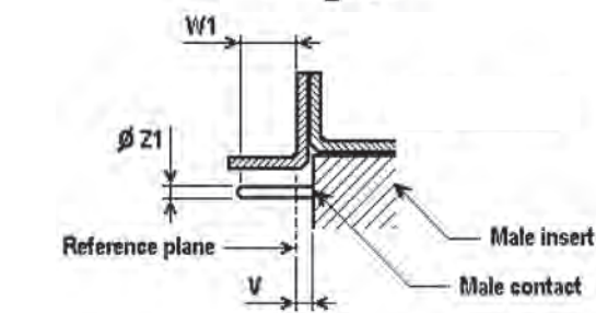
Male Connector
