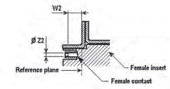
Female Connector
