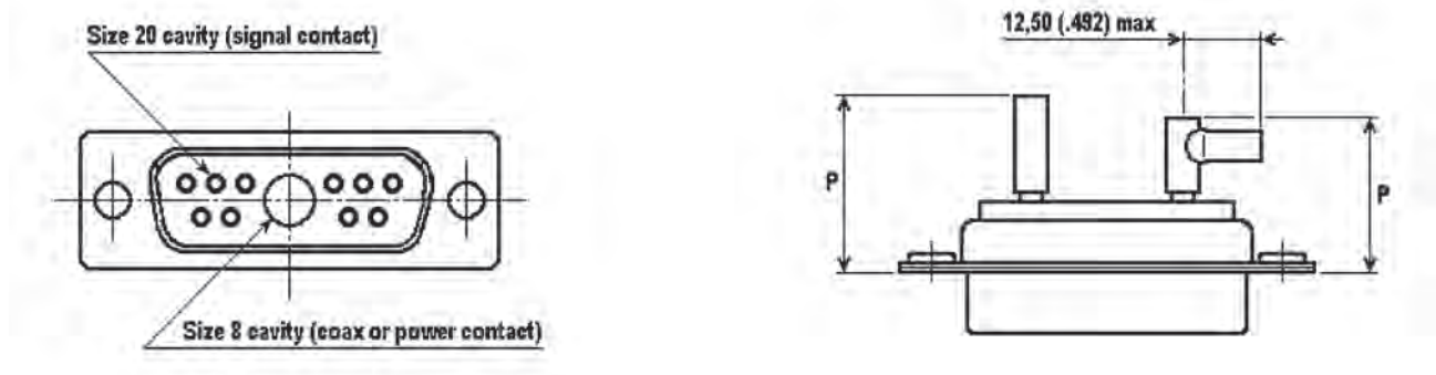
P max (Coaxial Contacts)
