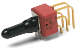
E221SD1AV2GE DPDT
