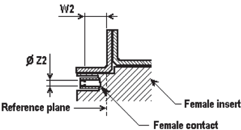
Female Connector
