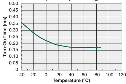
Typical Turn-On Time vs. Temperature ( I_F=5\text{mA} , I_L=100\text{mA}_{DC} )
