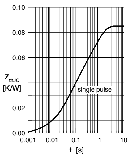
Fig. 7 Typ. trans. therm. impedance
