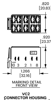
VC2 CONNECTOR HOUSING (For AMP terminals only)
