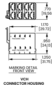
VCH CONNECTOR HOUSING
