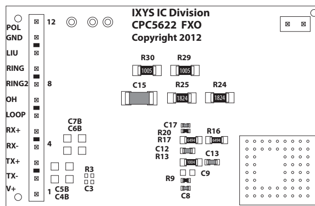
Figure 6. Bottom Side Components
